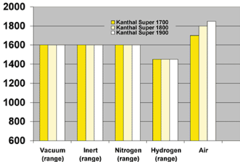
Figure 5. Maximum element temperatures for molybdenum disilicide elements in selected atmospheres.
